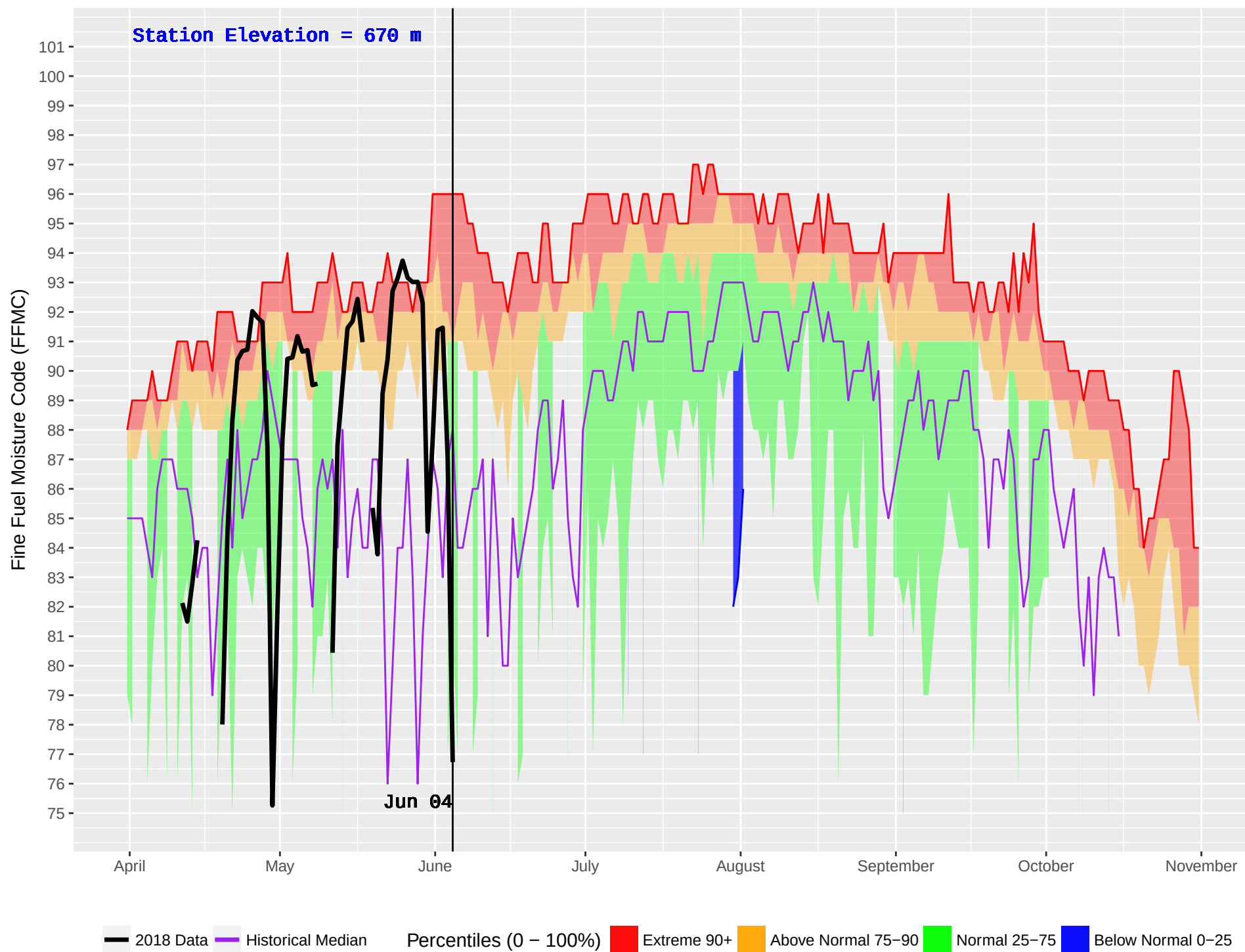
FINTRY (298) : Historical (1989–2016) and Current (2018) Noon Fine Fuel Moisture Code (FFMC)
