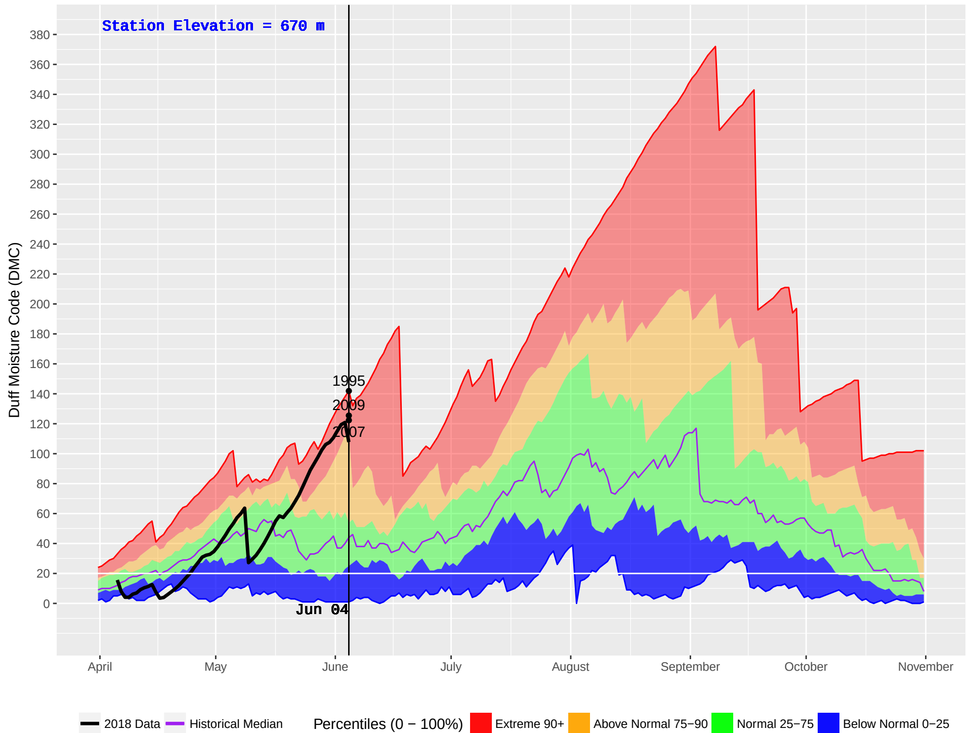
FINTRY (298) : Historical (1989–2016) and Current (2018) Noon Duff Moisture Code (DMC)
